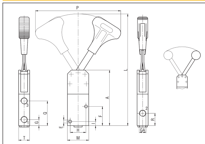
3/2 VERTICAL KNOB
