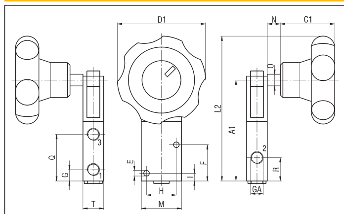
3/2 LATERAL HAND-WHEEL
