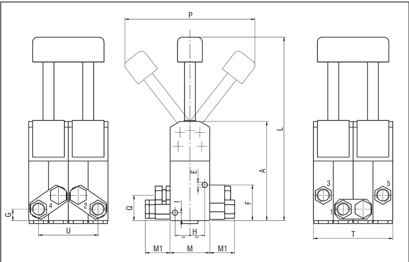
5/3 C.C. VERTICAL KNOB G 1/4 - G 1/2
