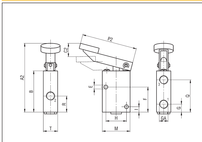
3/2 TAPPER
