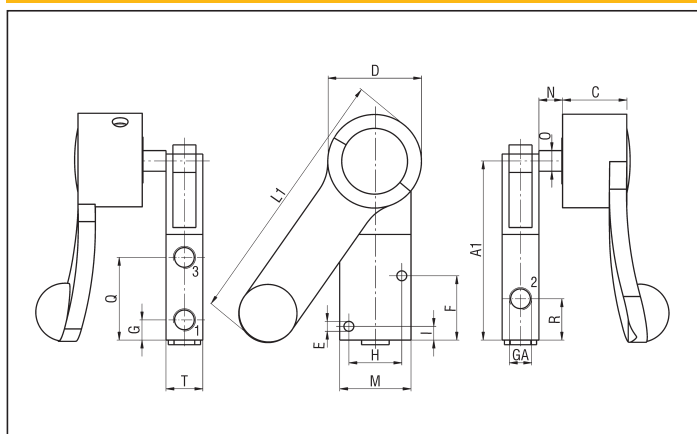
3/2 LATERAL KNOB
