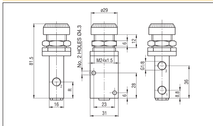
3/2 PUSH-BUTTON
