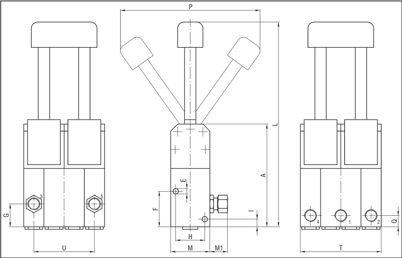
5/3 C.C. VERTICAL KNOB G 1/8
