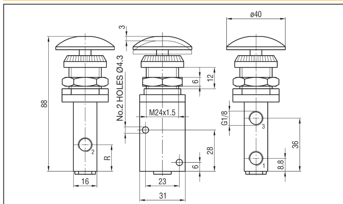
3/2 MUSHROOM
